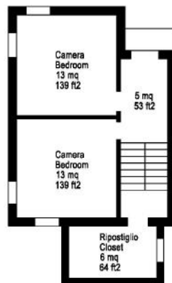
PIANO PRIMO FIRST FLOOR 0 1 2 3m 0 5 10ft
