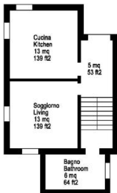
PIANO TERRA GROUND FLOOR 0 1 2 3m 0 5 10ft
