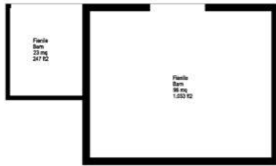
A EDIFICIO PRINCIPALE PIANO TERRA GROUND FLOOR 0 1 2 3m 0 3 10ft
